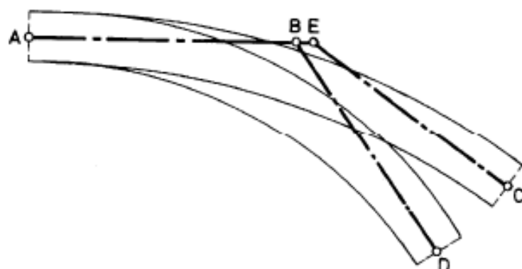
Figur 5. Sporskifteelement for i-krummet sporskifte.
